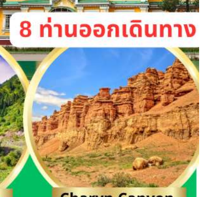
Charyn Canyon
